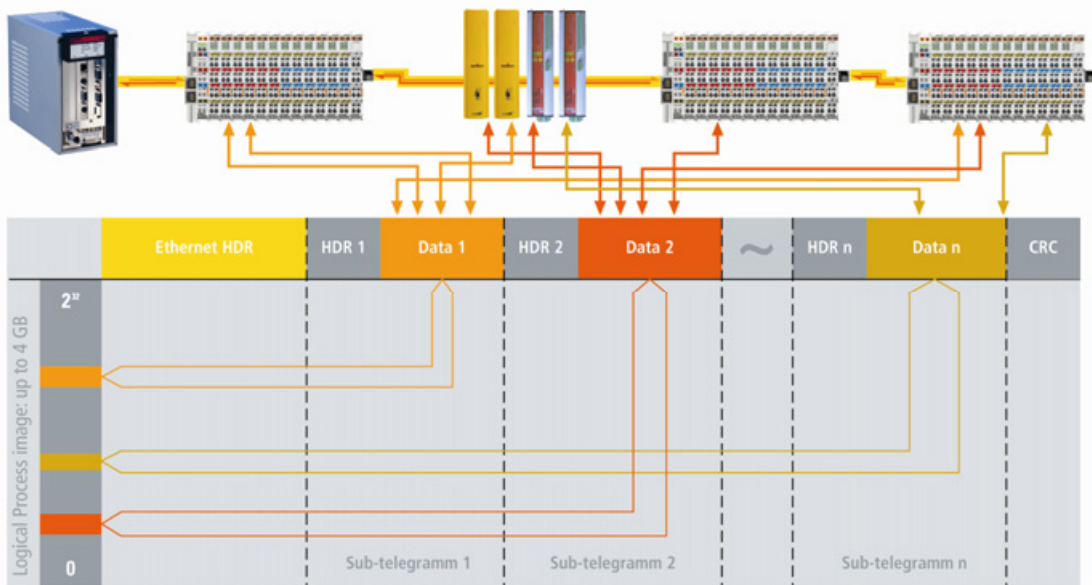
Figure 2: Process data is inserted in telegrams
