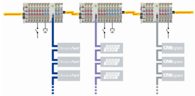
Figure 7: Decentralized Fieldbus Interfaces
