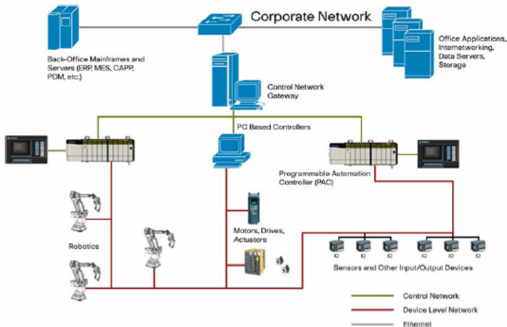
Figure 1: Traditional Proprietary Fieldbus Architecture
