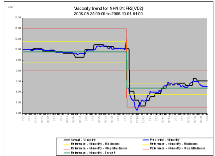
Figure 4- Monitoring against limits
